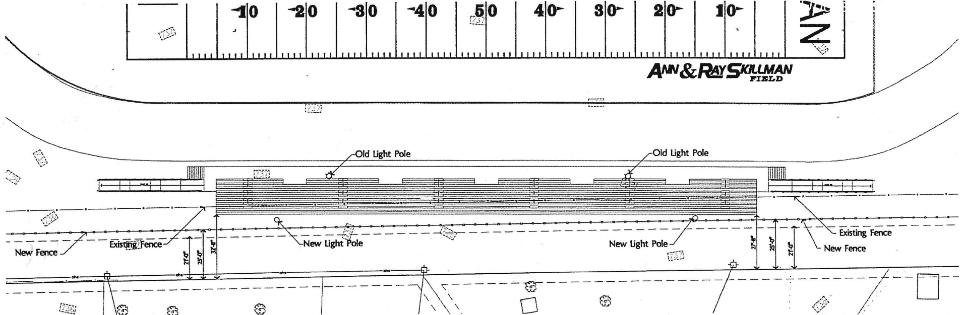
Bleacher Plan (1,400 Seats)
